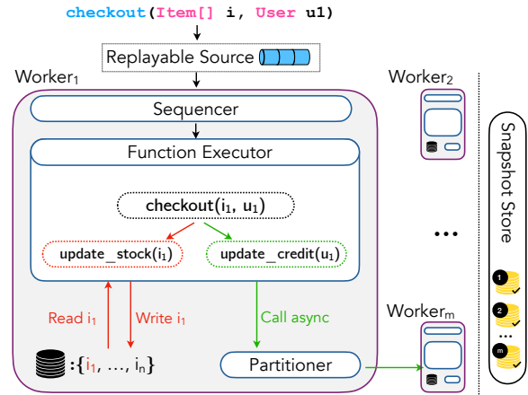
Figure 3: Stateful-Function execution in Styx.
