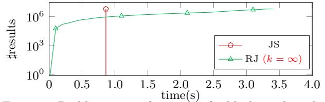
Figure 1: Problematic performance of a blocking algorithm and a representative top- k join algorithm using two TPC-H tables (cf., Table 3) and default settings (cf., Section 4).
