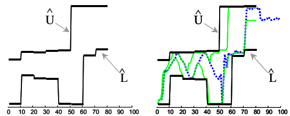
Figure 8. We can readily visualize \hat{U} and \hat{L} as the piecewise constant functions which bound, without intersecting, U and L , respectively. (Left) The \hat{U} and \hat{L} for the time series shown in Figure 5. (Right) The \hat{U} and \hat{L} shown overlaid on top of the generating time series.
