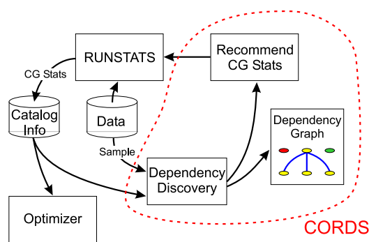
Figure 1: Role of CORDS in query optimization.
