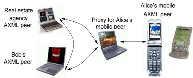
Figure 3: Outline of the demonstration configuration. process, e.g., agency's owner or client workspaces.
