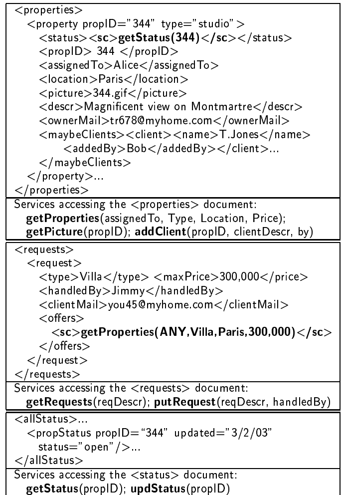
Figure 2: Workspace for the real estate agency
