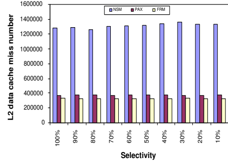
Figure 11: Data cache penalty of NSM/PAX/FRM with one selected attribute
