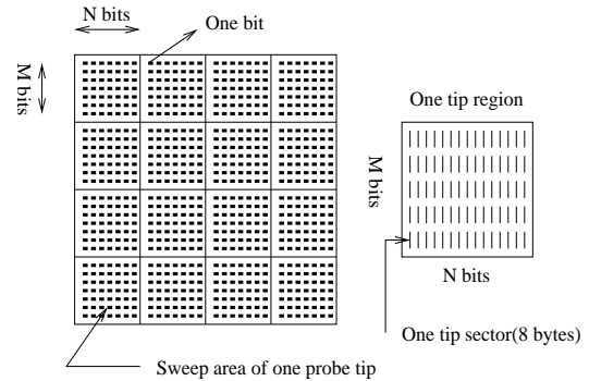
Figure 2: The media sled organization
