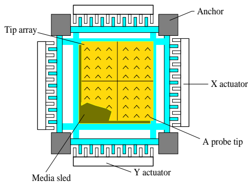
Figure 1: The architecture of CMU CHIPS
