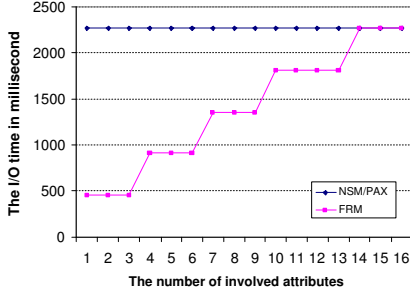
Figure 10: Comparison of I/O time for NSM/PAX/FRM
